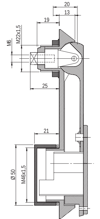
Swinghandle HS 01 rectangular MATERIAL: Housing - PA 6 GF30; black, white, grey RAL.
