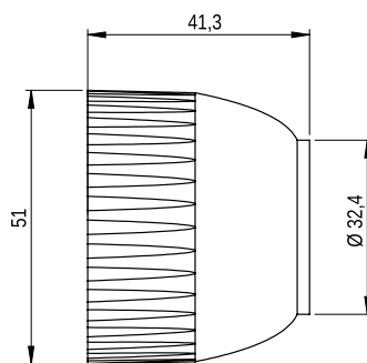
Insulator
