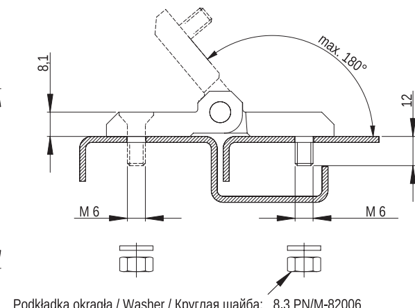
Hinge P60/J
