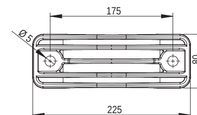
Cable Clamp KO 132
