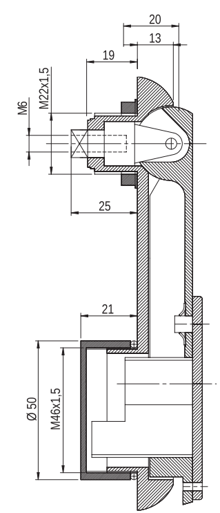
Swinghandle HS 01 MATERIAL: Housing - PA 6 GF30; black, white, grey RAL.
